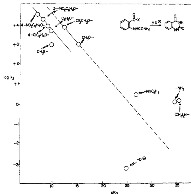
Figure 7. Plot showing dependence of the log of the second-order rate constants for hydroxide ion catalyzed cyclization ( l. mol^{-1} sec^{-1} ) of indicated compounds upon the pK_a values of the conjugate acid of the leaving groups ( -X ).
