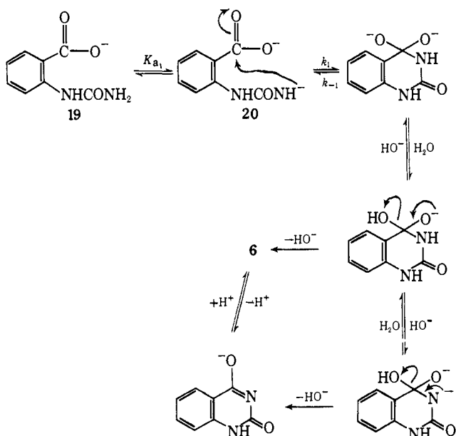
Scheme V
