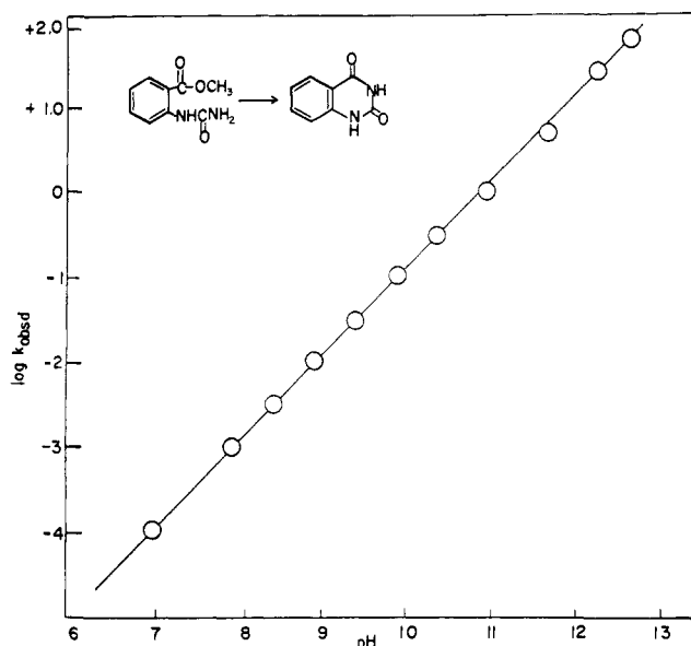
Figure 1. pH- \log k_{\text{obsd}} profile for 5 \rightarrow 6 (30°, \mu = 1.0 , H 2 O; rate constants in units of sec -1 ).
