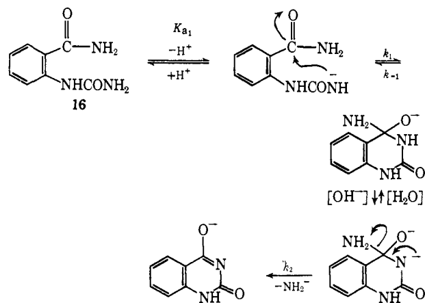
Scheme VII
